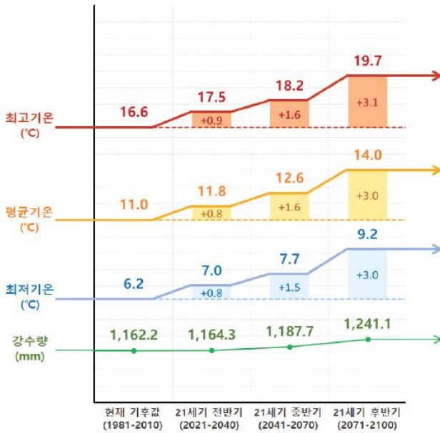
RCP6.0
