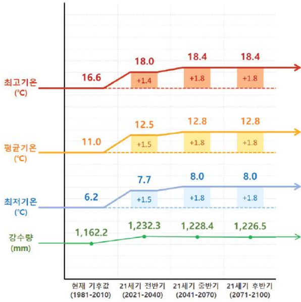
RCP2.6
