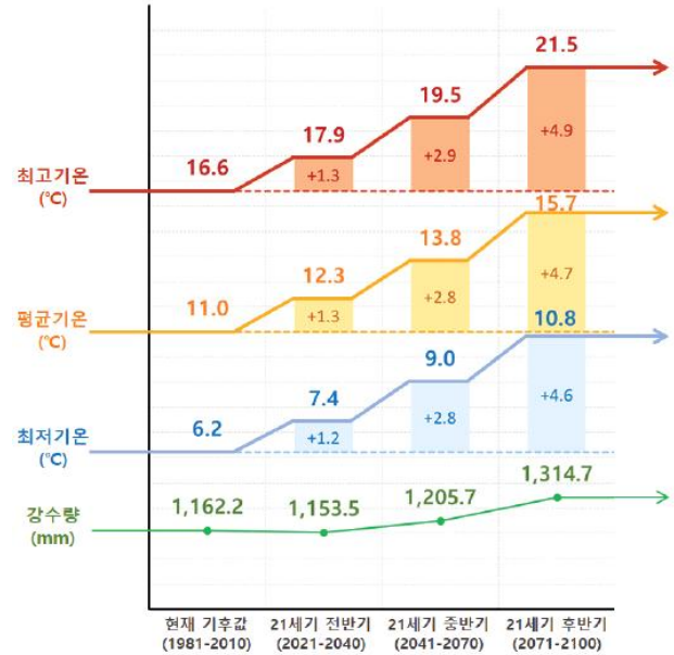
RCP8.5
