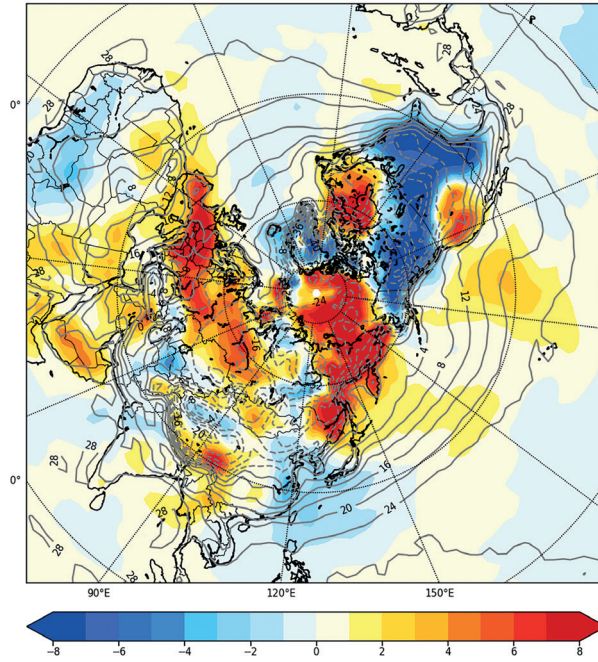
2m TM Mean anomaly by NCEP R1 with norm(1991~2020) [2022.12.20~2022.12.26]
